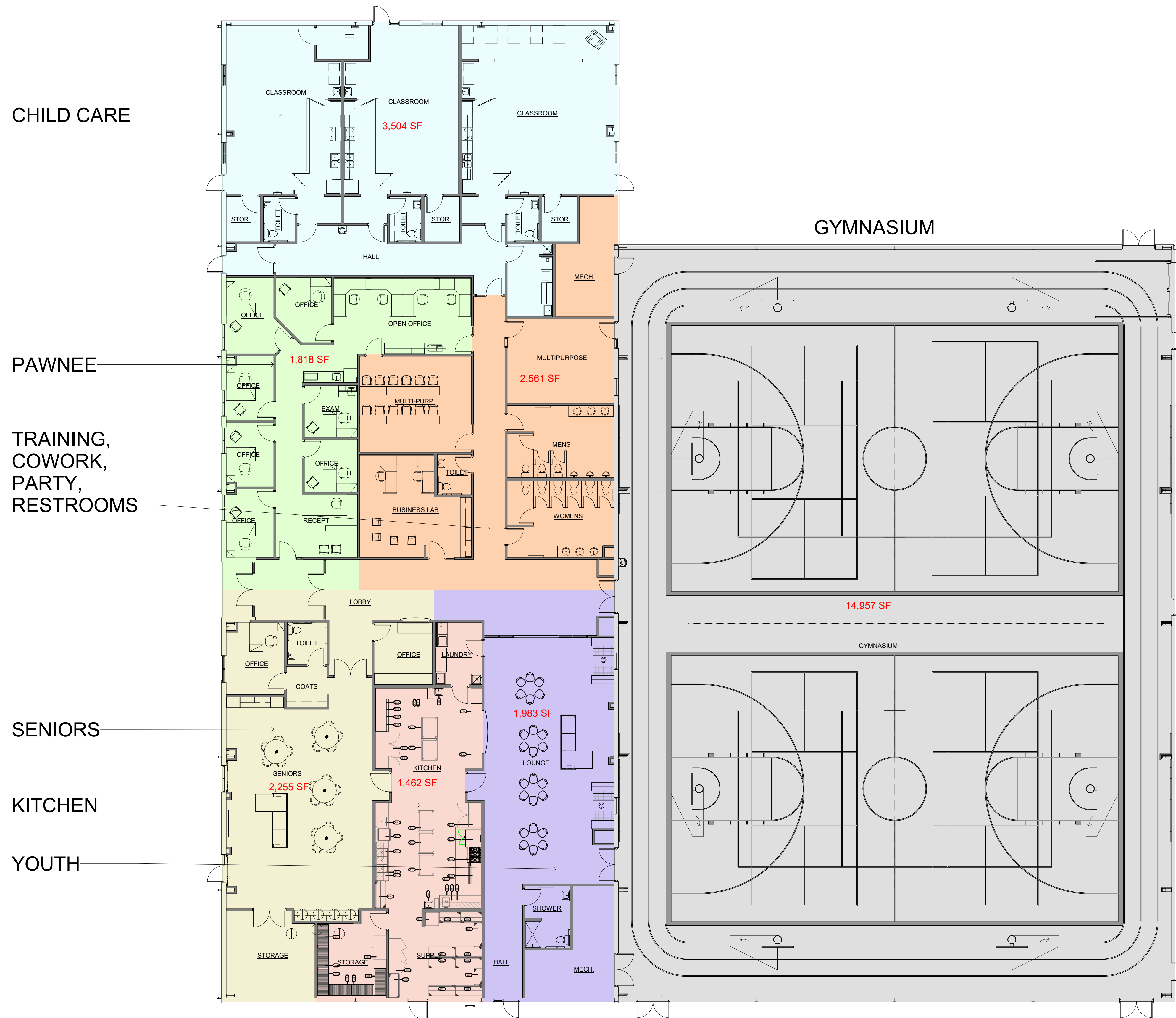
1 OVERALL FLOOR PLAN 3/32" = 1'-0" 28,540 SF TOTAL
