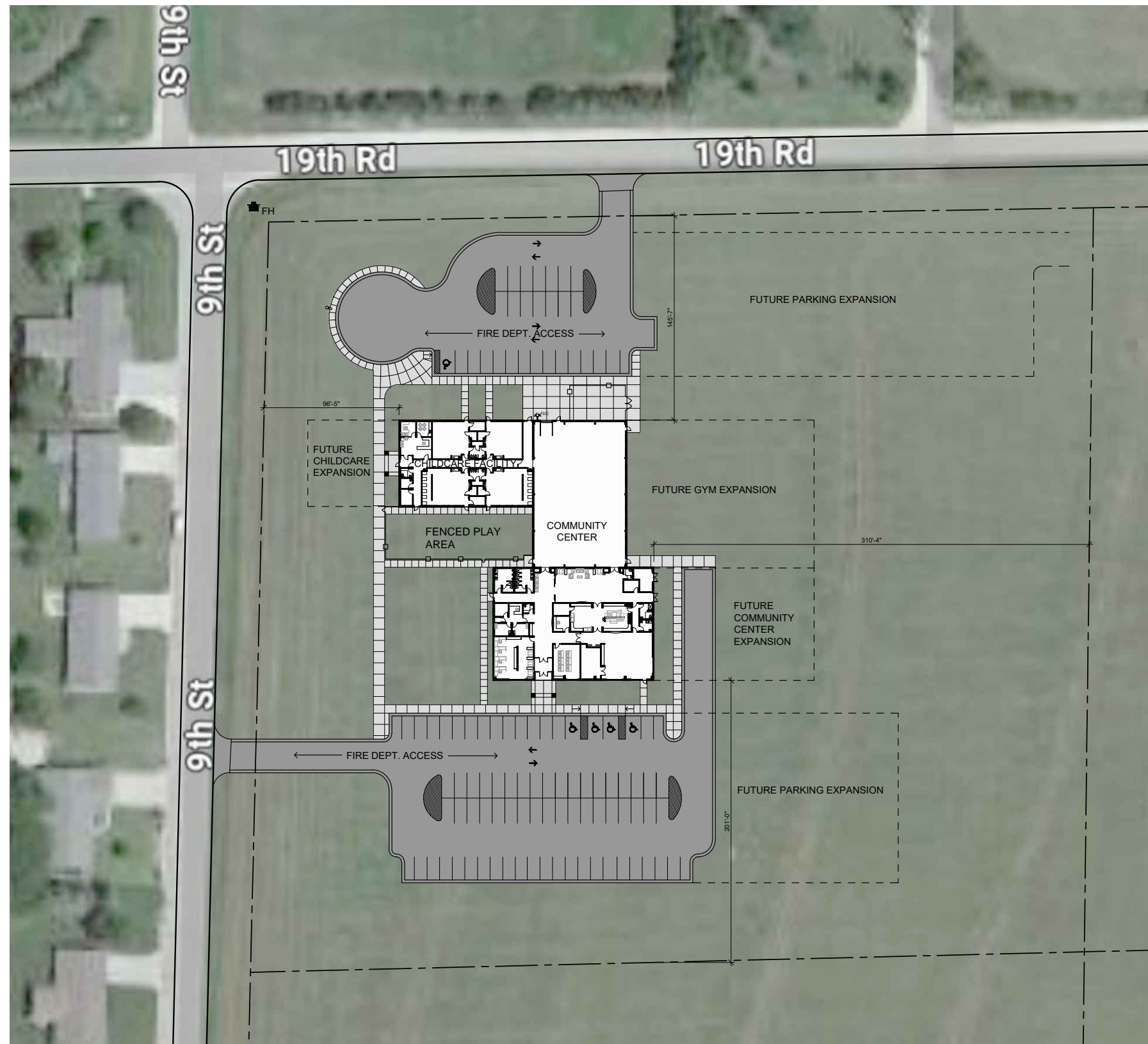
1 SITE PLAN 1"=40' 0 40'
